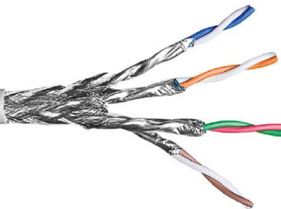
ASIAWIRE Cat.6A S/FTP 23WAG LSZH 4P Cable
